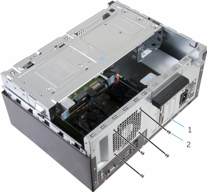
1 chassis
